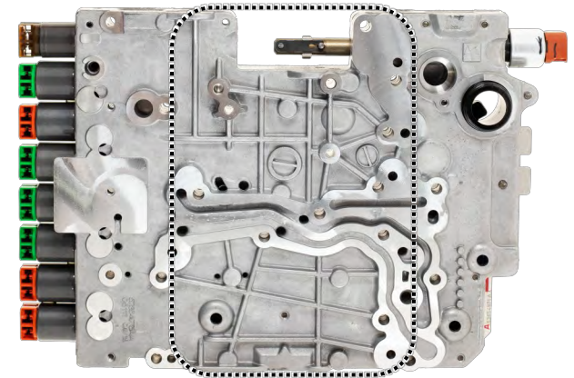
GEN2 no valves in upper casting.
