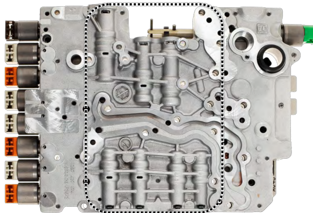
GEN1 has valves in upper casting.
