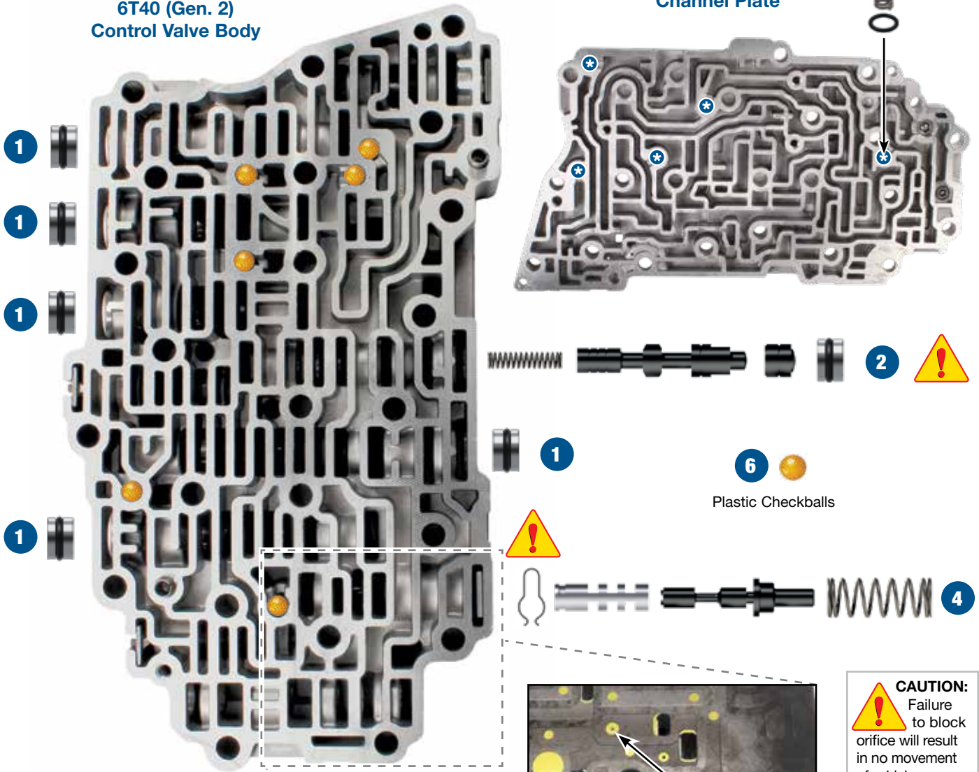
6T40 (Gen. 2) Channel Plate
