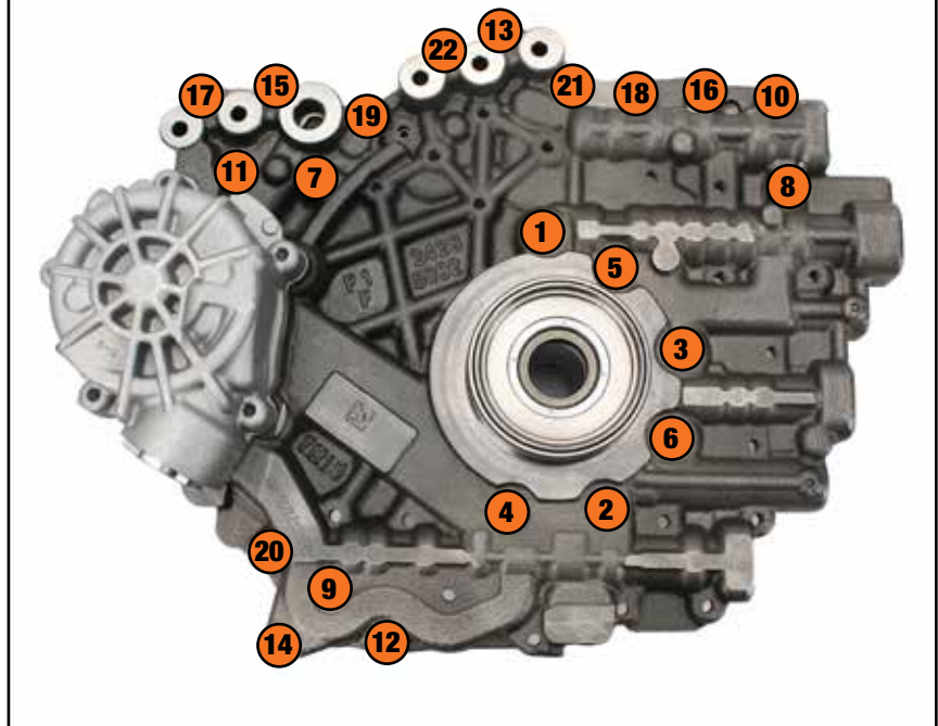
GM 9T50 Pump Body
