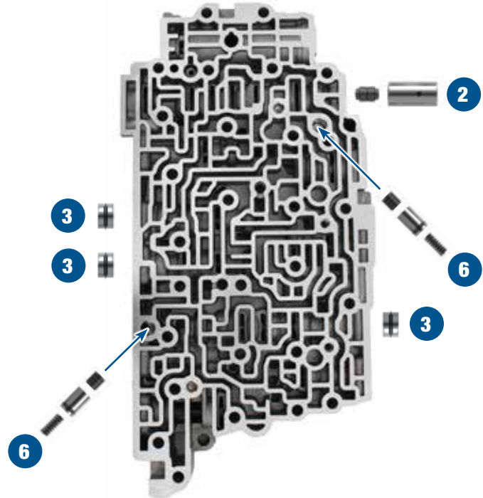
9T50 Main Control Valve Body
