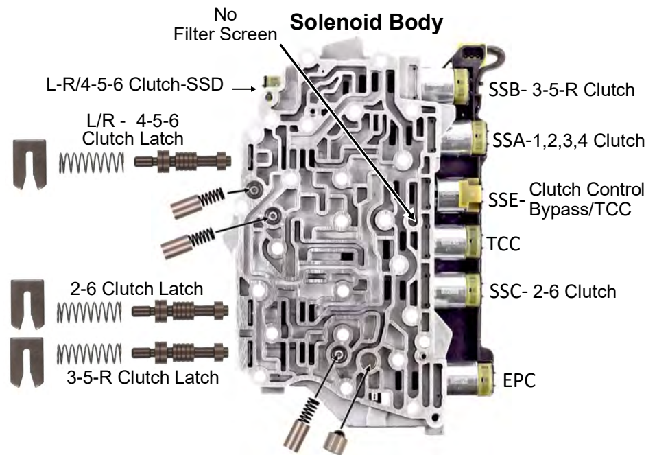
Solenoid Body Plate
